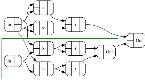
Figure 8: magSqr in D_{Cont_{(-\rightarrow)}}^{\mathbb{R}}
