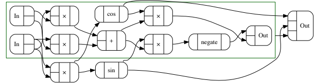
Figure 5: \hat{D} cosSinProd
