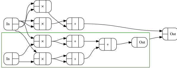
Figure 4: \hat{D} magSqr
