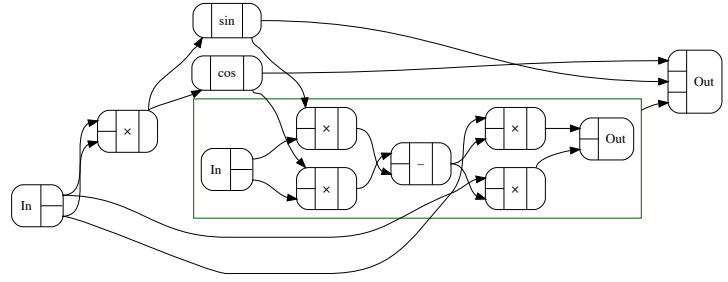
Figure 9: cosSinProd in D_{Cont_{(-\rightarrow)}}^{\mathbb{R}}
