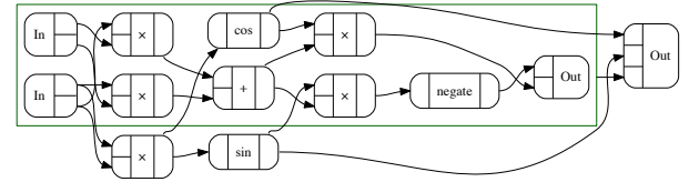
Figure 5: \hat{D} cosSinProd
