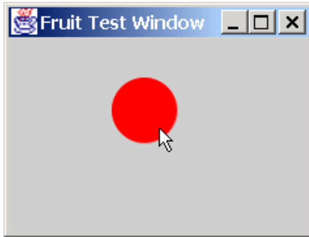
Fig. 1. Running ballGUI
